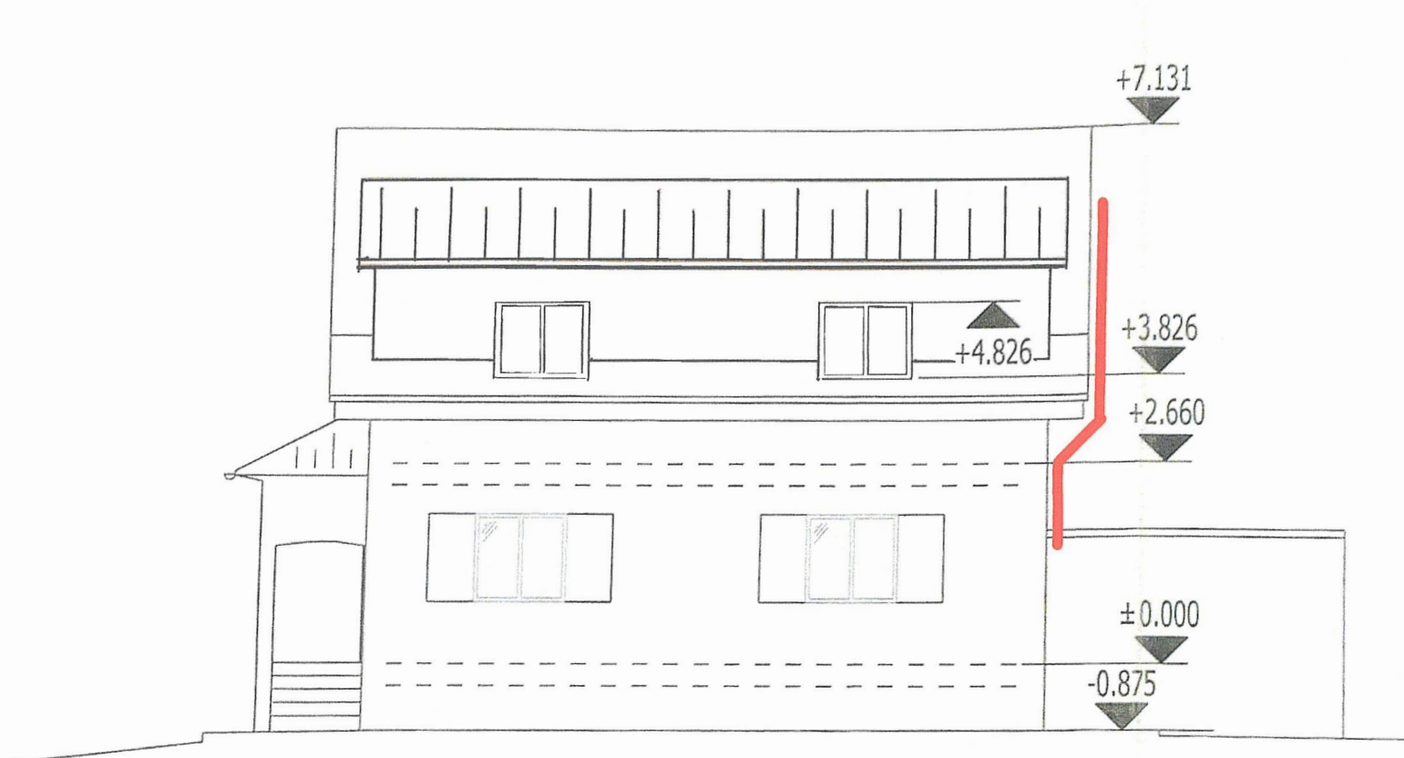
West Fassade
